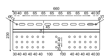
Figure 3.6 - Pitched roof load distribution plate (Cod. 000224 ) for PBS device
