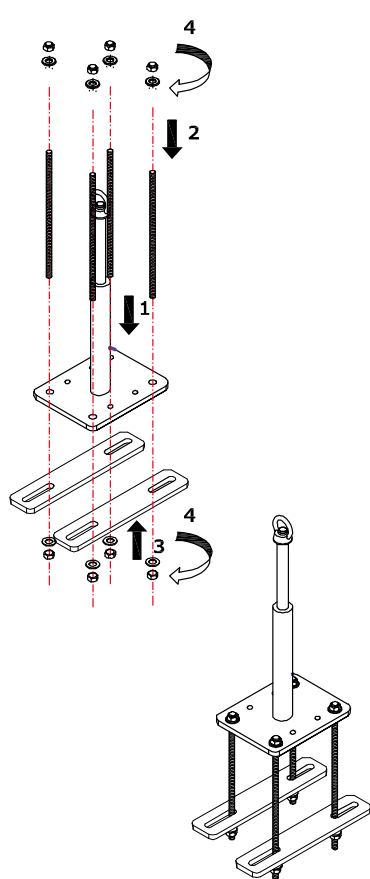
Figure 3.15 - Device PBS/PBSC with counterplates (Cod. 000039)
