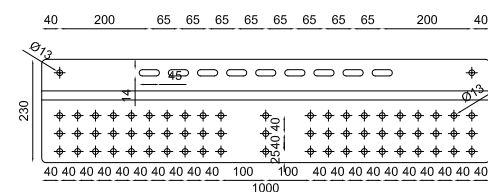
Figure 3.5 - Pitched roof load distribution plate (Cod. 000220 ) for PBS device
