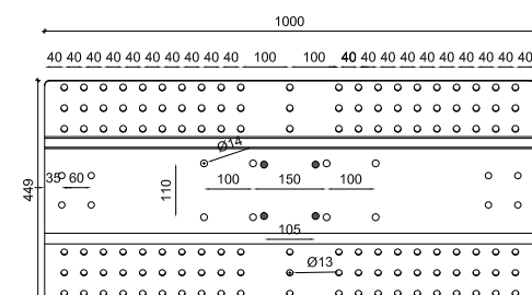
Figure 3.3 - Ridge beam load distribution plate (Cod. 000218 ) for PBS device
