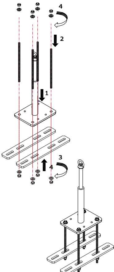
Figure 3.16 - PBS/PBSC device with counterplates (Cod. 000203)
