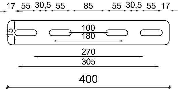
Figure 3.13 - Galvanised steel counterplate (Cod. 000203) for devices PBS/PBSC
