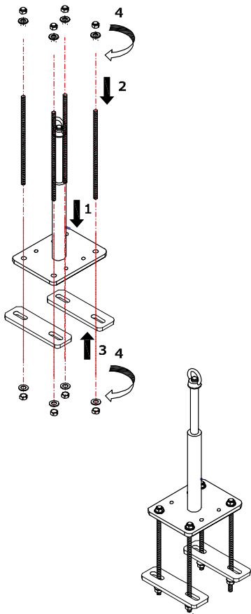
Figure 3.14 - Device PBS/PBSC with counterplates (Cod. 000196)
