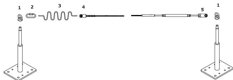
Figure 5.2 - Single span lifeline
