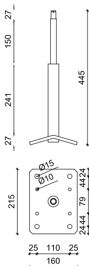
Figure 3.2 - Potelet PBSC
