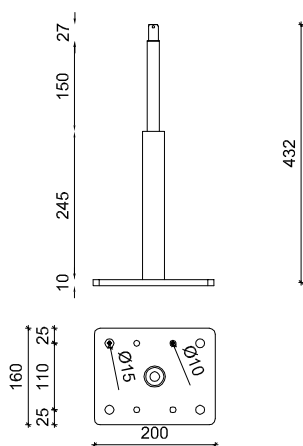
Figure 3.1 - Potelet PBS
